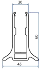
GP 6043 60x43 Cam Kanallı Gemici Profili 60x43 Glass Channel Profile
